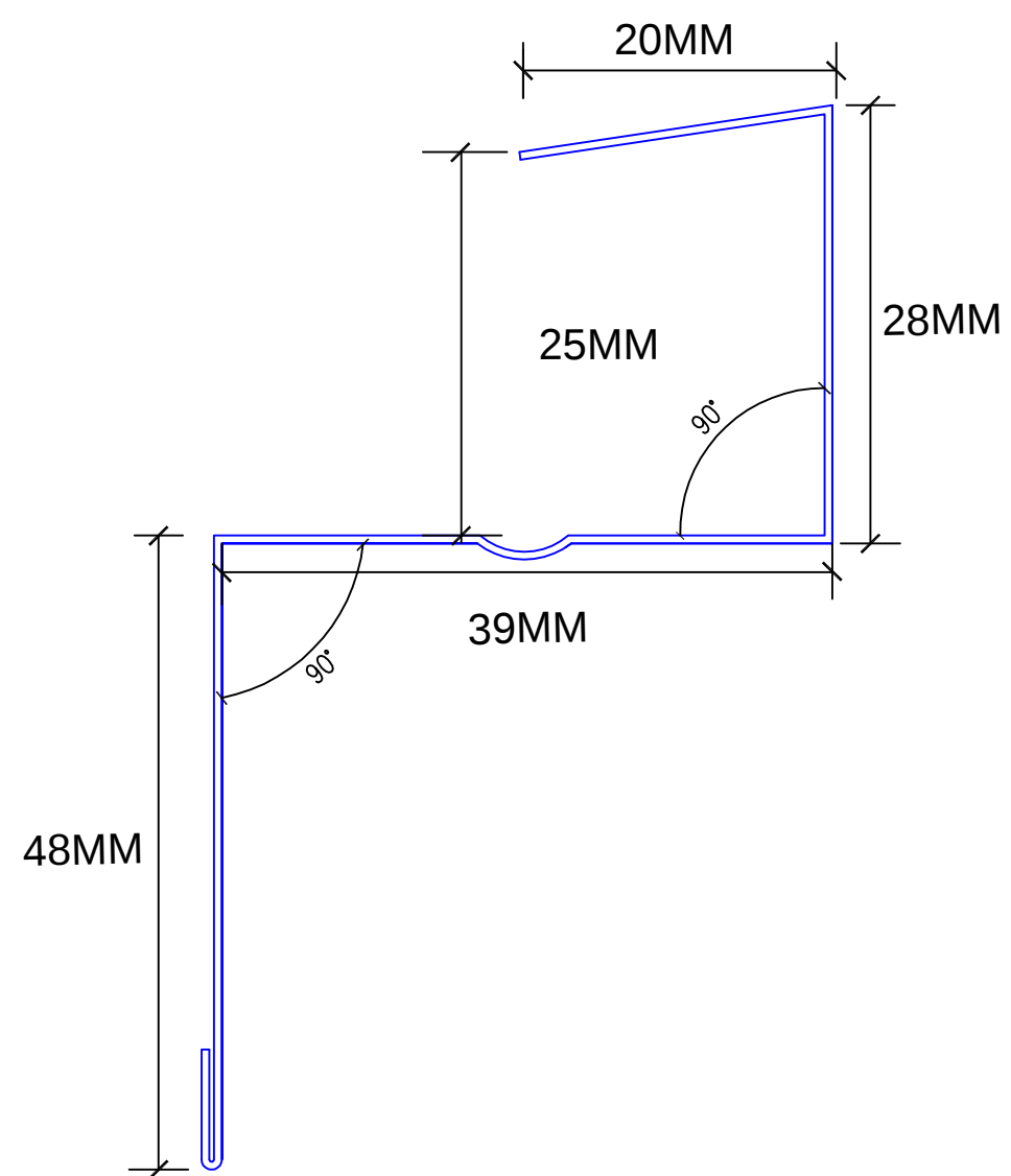
C03N - EXISTING NATURAL SLATE TRIM TYPE 3 ALUMINIUM Length 3050mm
